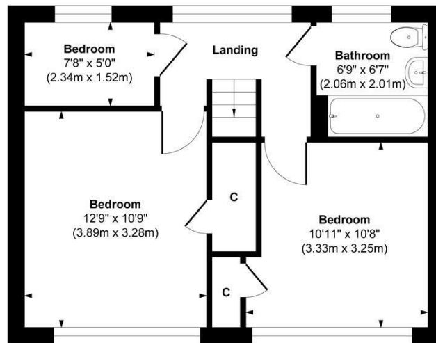
First Floor Approximate Floor Area 429 sq. ft (39.85 sq. m)
